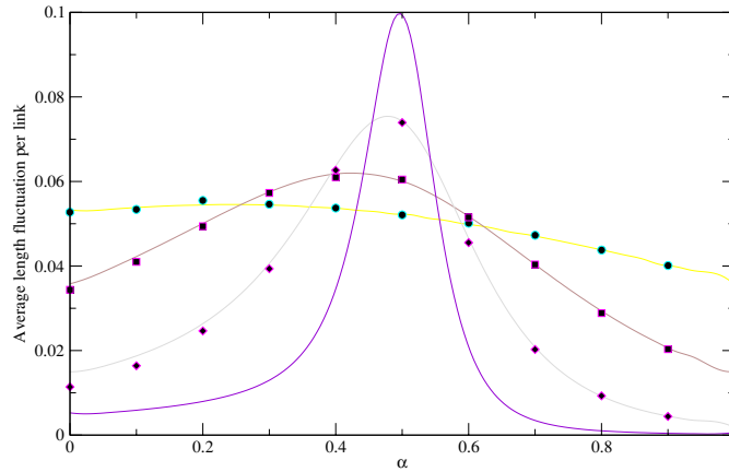
Figure 2. The average per link length fluctuations (1/N)\langle(H_L - \langle H_L \rangle)^2\rangle for the centred TSP according to the formalism of [4] shown for \beta = 2.0, 5.0, 10.0, 20.0 with increasingly pronounced peak. Points (omitted at \beta = 20.0 ) are from Monte Carlo simulations with N = 1000 averaged over 100 random instances.
