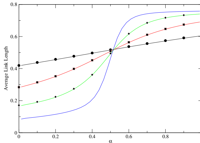
Figure 1. The average link length (1/N)\langle H_L \rangle for the centred TSP according to the formalism of [4] shown for \beta = 2.0, 5.0, 10.0, 20.0 with increasingly sharp step. Points (omitted at \beta = 20.0 ) are from Monte Carlo simulations with N = 1000 averaged over 100 random instances.
